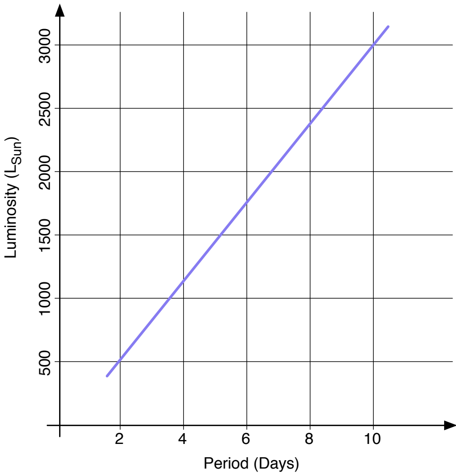
Luminosity vs Period for Cepheid Variables
